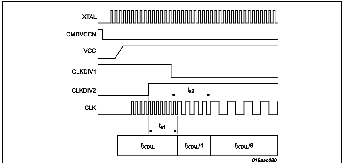
Fig 24. Unwanted frequency during the switch
